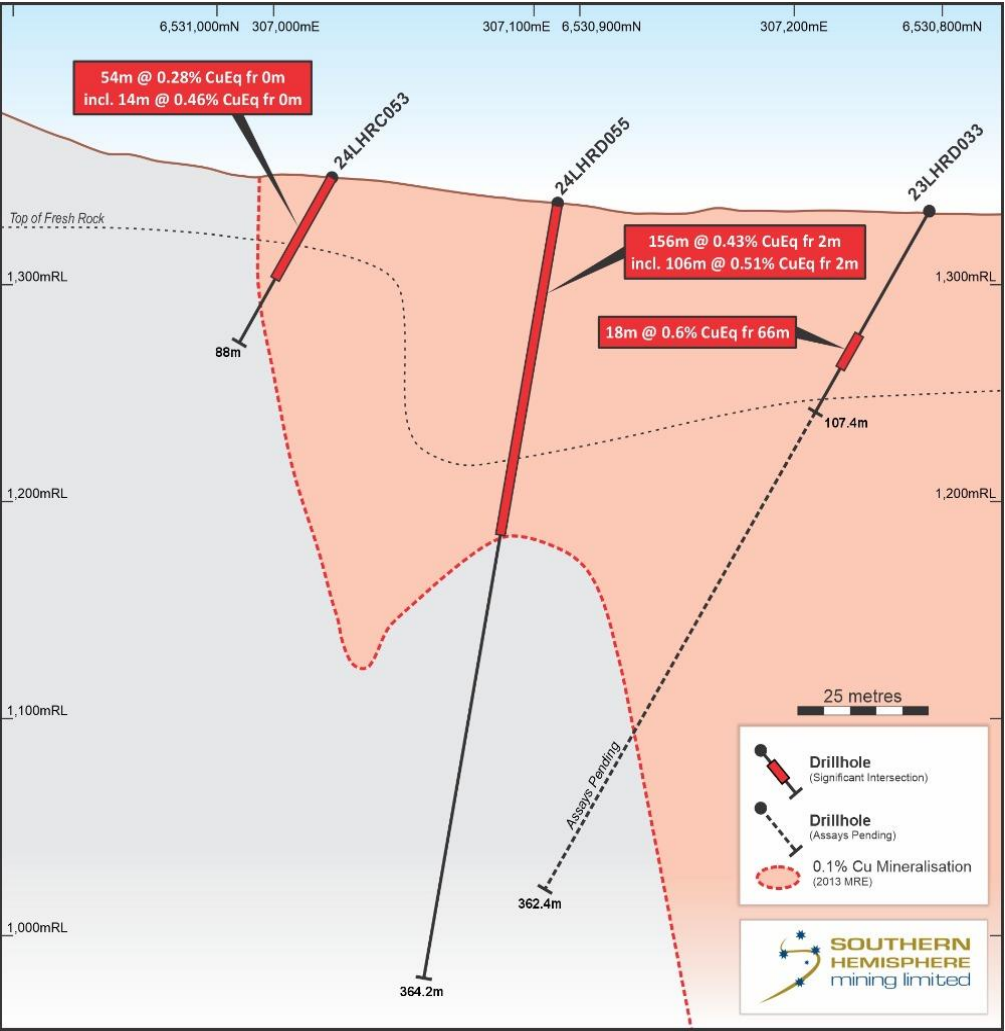
Cerro section of hole 24LHRD055
