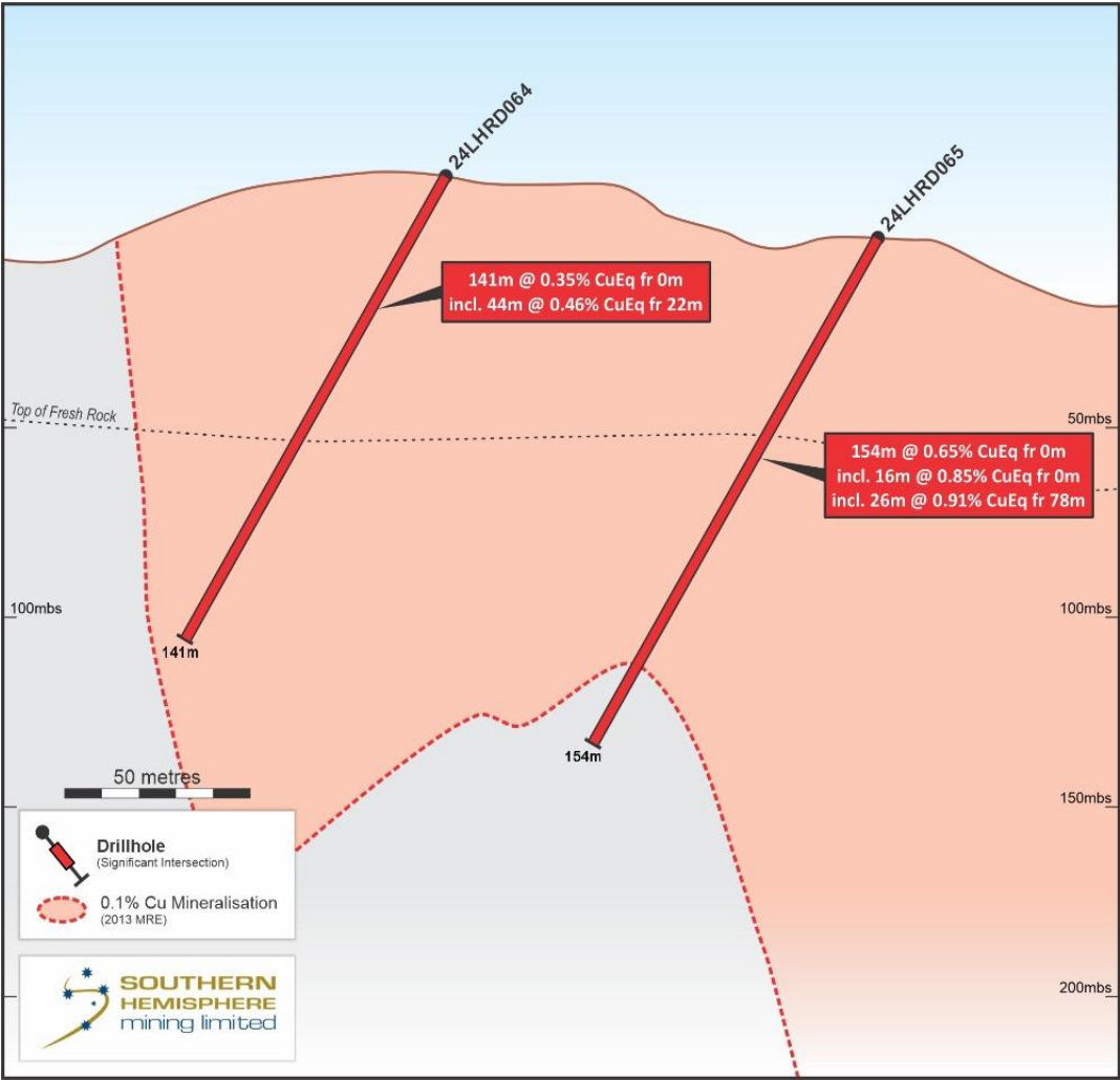
Cerro Section with holes 24LHRD064 and 24LHRD065.
