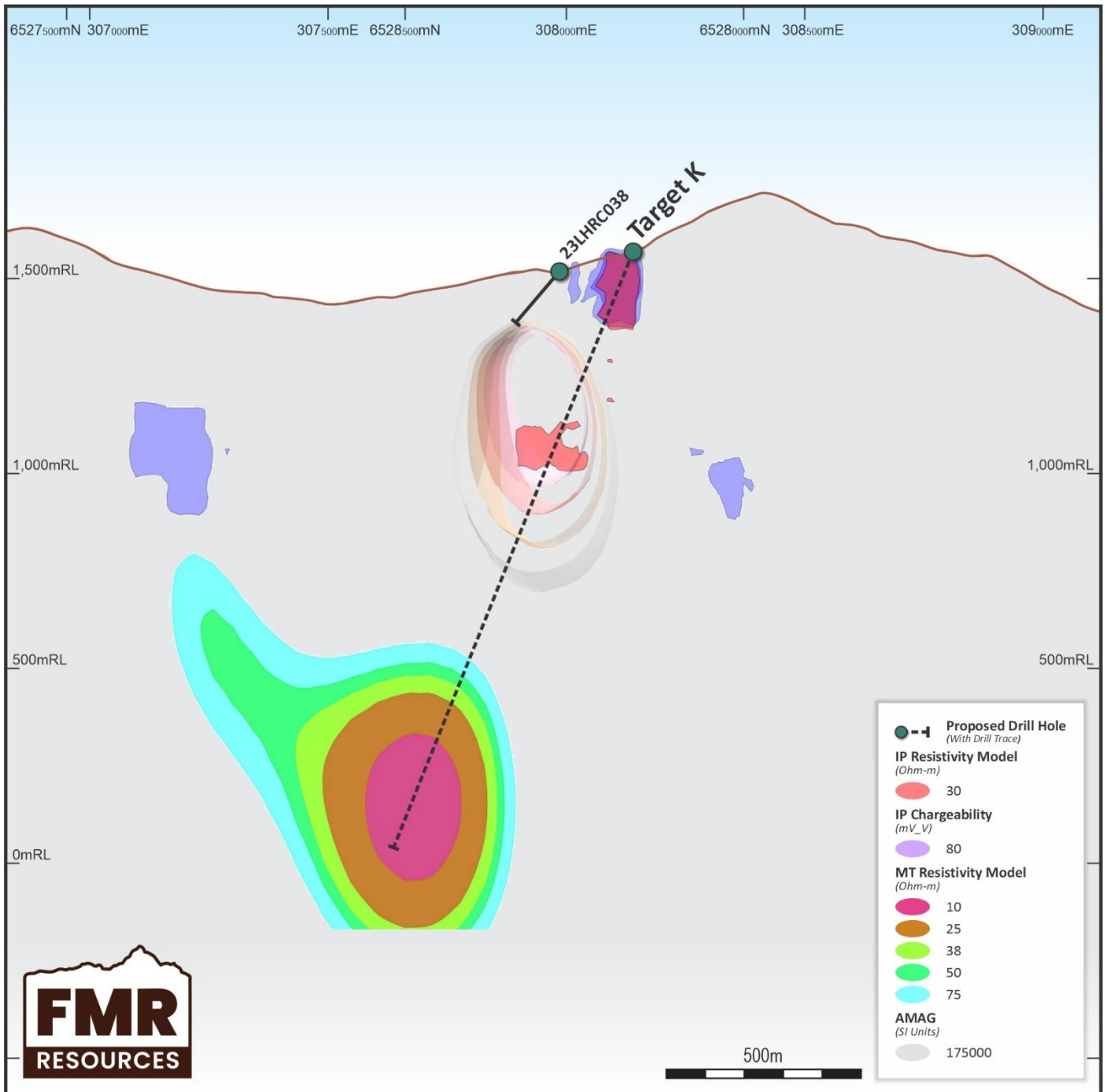
Figure 2. Cross section K-K', Target K, showing geophysical models and proposed drillhole to 1,650m downhole depth, testing relatively shallow IP-RES and IP Chargeability features interpreted to be related to the Santa Maria epithermal vein system, and a large MT high amplitude feature at depth (+/- 10m window).
