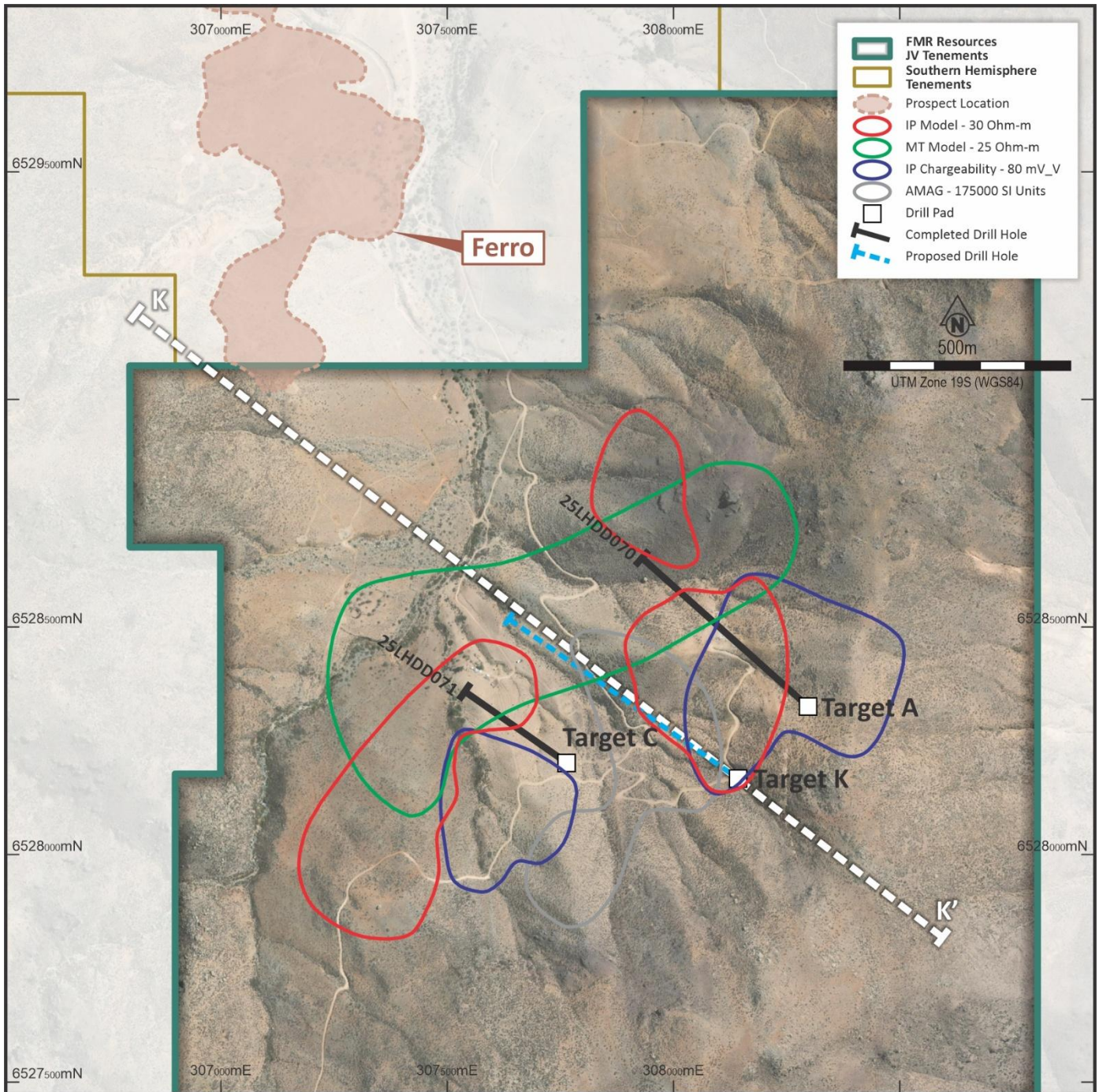
Figure 1. Plan view of Southern Porphyry, showing surface projections of geophysical models, mapped epithermal veining at surface, and completed and planned drill targets.
