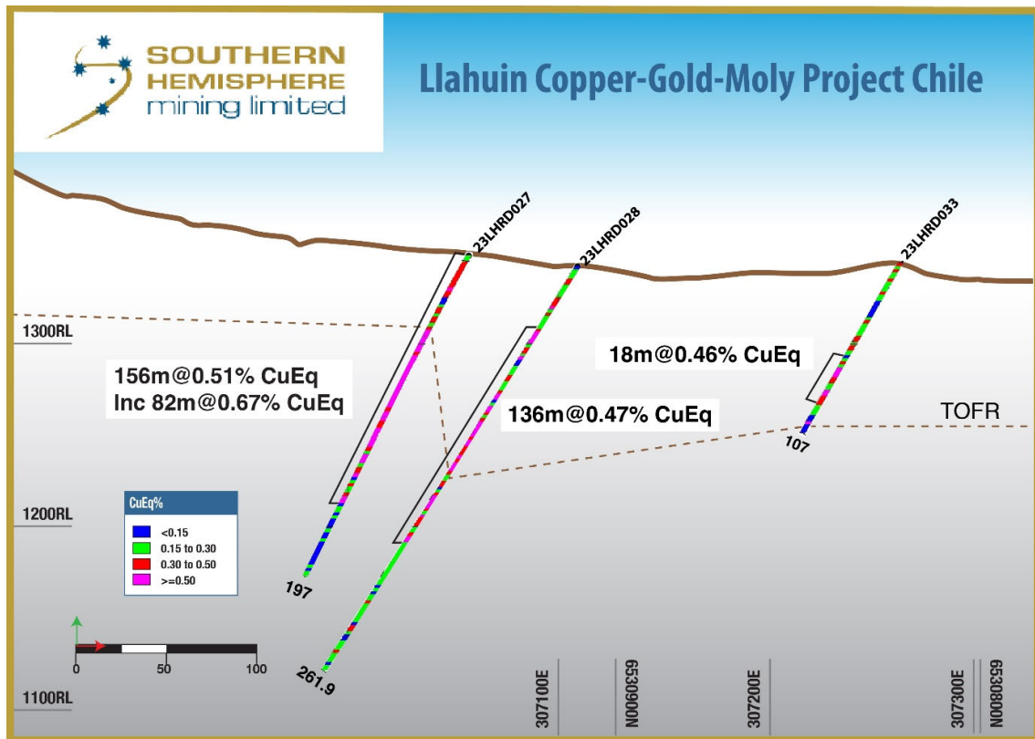
Figure 3. Cross section through 23LHRD027, 23LHRD028, and 23LHRD033, showing reported intercepts. Note that historical holes are omitted from the cross section for the purpose of clarity, as they are oblique to the section, at a sub optimal angle to interpreted mineralisation.
