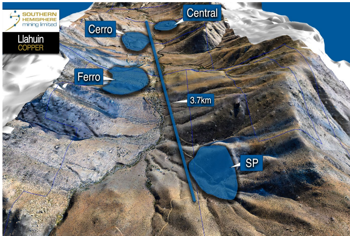
Figure 5. 3D view looking northeast from Southern Porphyry (SP) to Central Porphyry, showing the scale of the Llahuin mineralising system.
